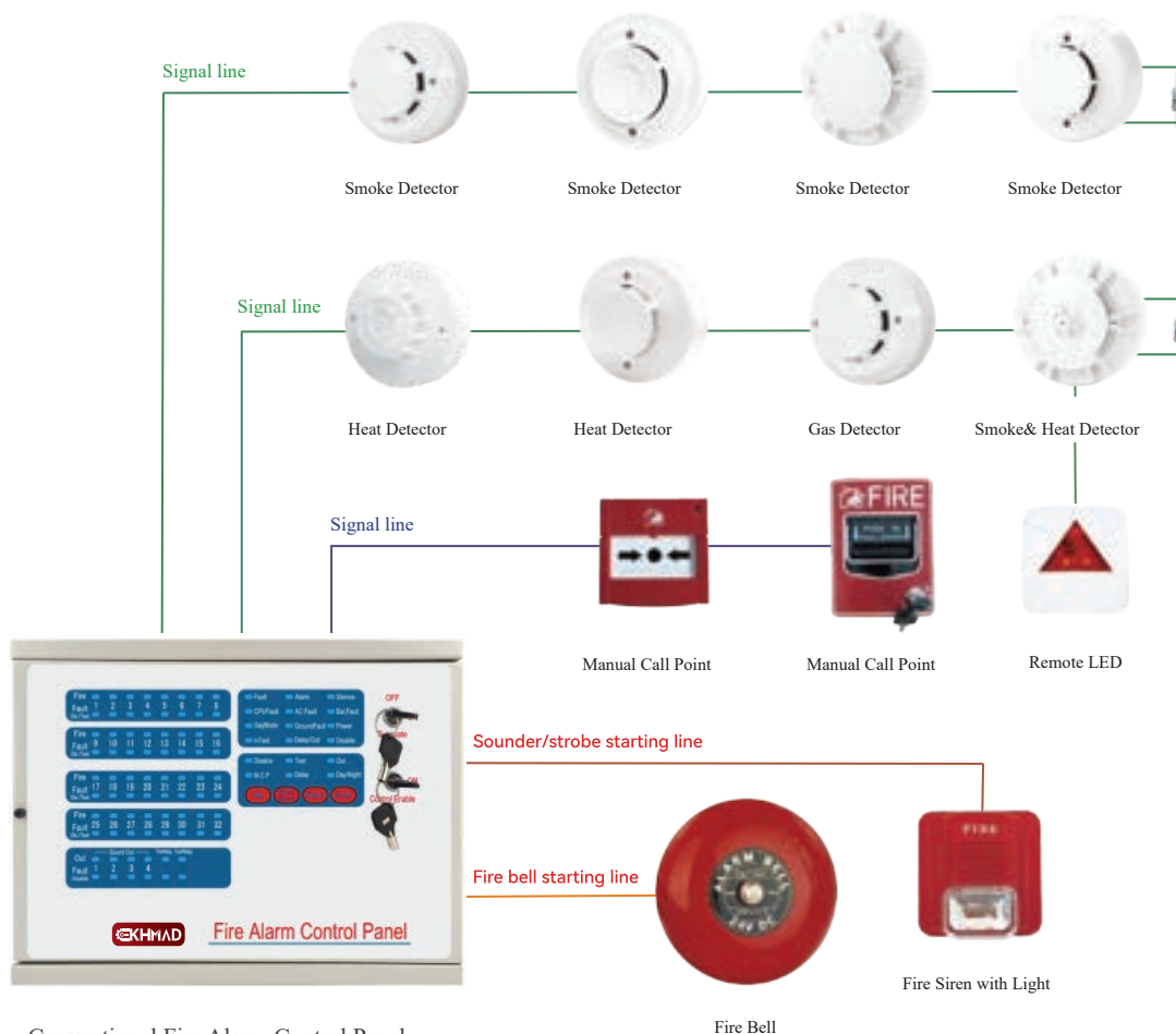
Conventional Fire Alarm Control Panel
